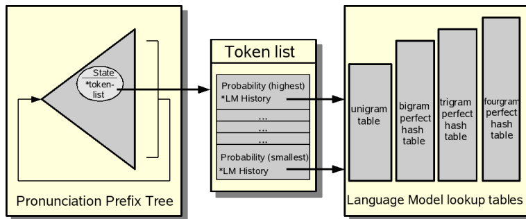
Figure 3: The decoder uses a single Pronunciation Prefix Tree (PPT) and a 4-gram Language Model (LM). Each HMM state from the PPT can contain a sorted list of tokens. Each token from a list has a unique LM history.
