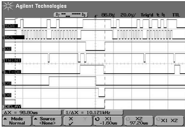
Figure 7. A screenshot of the oscilloscope displaying TWI bus data.
