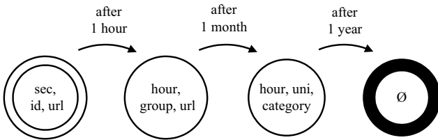
Figure 2: Example of a degradation policy noted as a DFA
