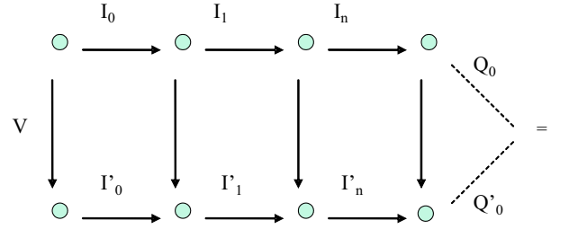
Figure 3: After n inserts I in the original database, a query Q on this data should return the same result as an alternative query Q' on n degraded inserts I' .
