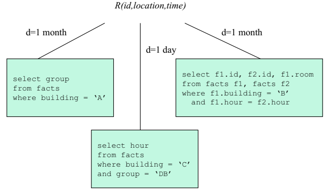
Figure 4: Three queries are specified on a relation R(id,location,time) and retention periods \delta after which the data should be removed such that it will not be part of the query answer anymore.
