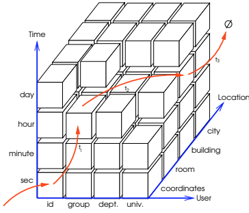
Figure 1: The different domain generalization graphs together form a cube. A Life-Cycle Policy is a set of transitions between elements (states) of this cube and the events which trigger the transitions.
