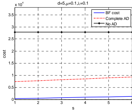
Figure 7 The impact from change of s ( d = 5 , \lambda = 0.1 )
