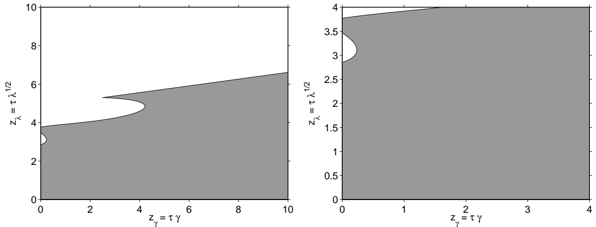
Figure 4: Stability region (shaded area) of the fourth-order local Richardson extrapolation (25). The right plot zooms in on the region where stability for wave term z_\lambda is guaranteed. Stability for the conduction term z_\gamma is unconditional.
