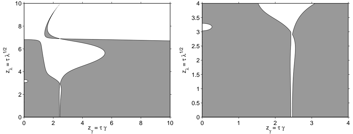
Figure 3: Stability region (shaded area) of the fourth-order composition method. The right plot zooms in on the region where stability is guaranteed. (Cf. Figure 5.1 in [10].)
