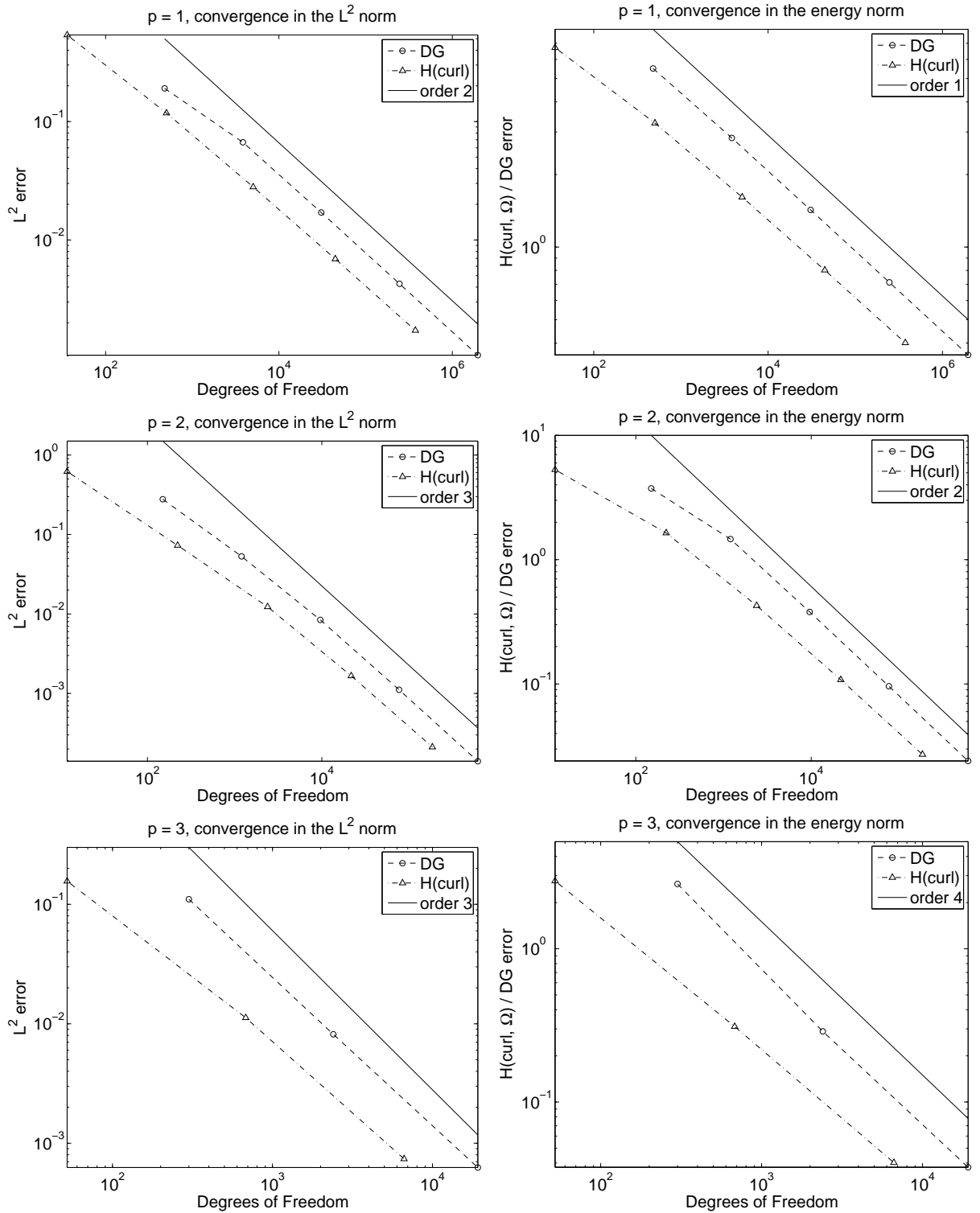
Figure 5: Convergence plots in the L^2 -norm (left column) and in the energy norm (right column) for test example (27) with \sigma = 60\pi . In each plot the convergence rates of the DG method and the H(\text{curl}) -conforming method are shown along with the expected order of convergence.
