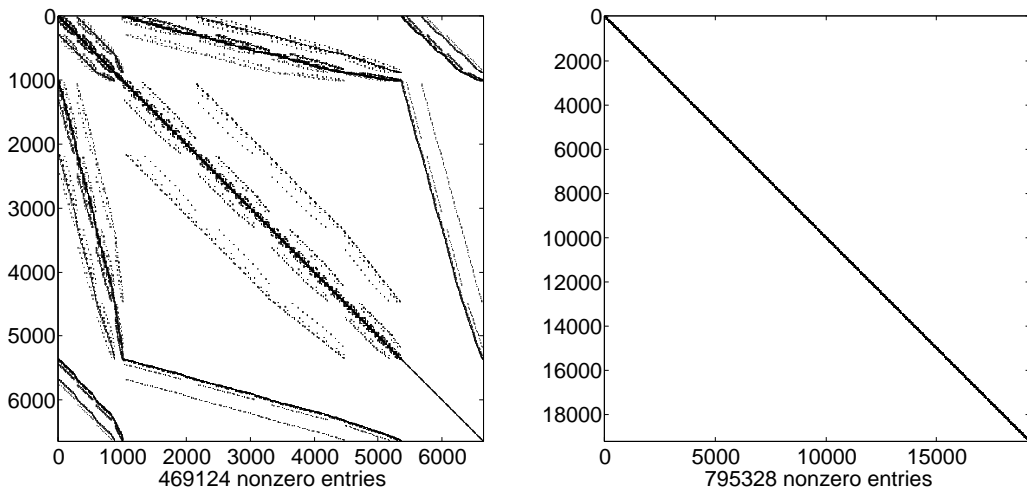
Figure 1: Sparsity pattern of the mass matrix for H(\text{curl}) -conforming FEM (left) and DG-FEM (right) for a mesh with 320 elements. Third-order polynomials are used, which means that the size of the blocks in the right plot is 60 \times 60 . Note the difference in size between the two matrices.
