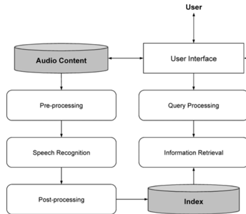
Figure 1: A generic spoken document retrieval system.
