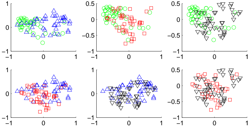
Figure 1: Visualization of the first two principle components of all six possible combinations of two emotion classes. The emotion classes are plotted per two to facilitate the visual inspection. The plots illustrate how difficult it is to separate even two emotion classes, where separating four emotion classes is the aim.
