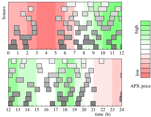
Fig. 5. Schedule of scenario 3
