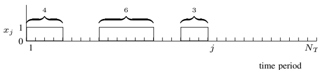
Fig. 1. A possible representation of state (3,13,2)
