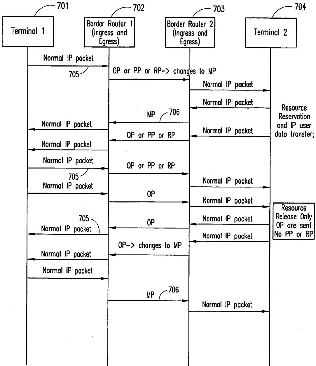
Resource reservation and resource release procedures in Load Control
