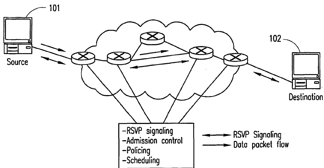
RSVP/Intserv framework
