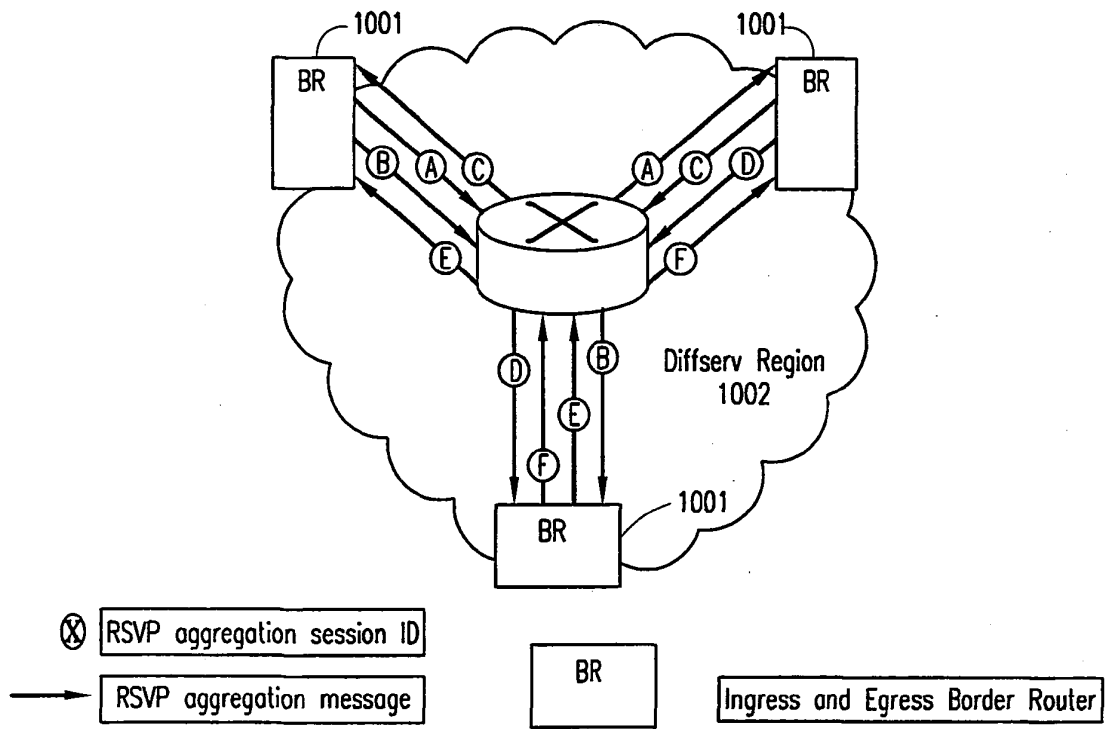
Example of full meshed Diffserv domain with three Border Routers and one Core Router
