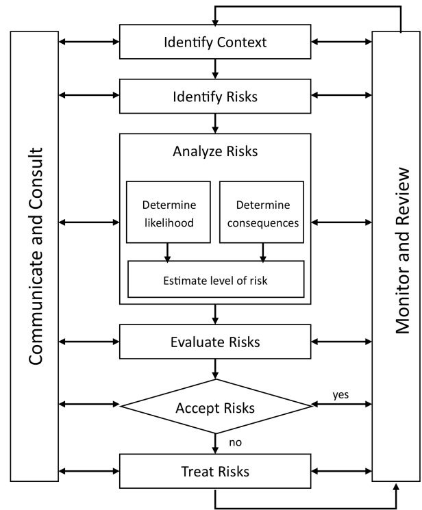
Fig. 2. CORAS sub-processes
