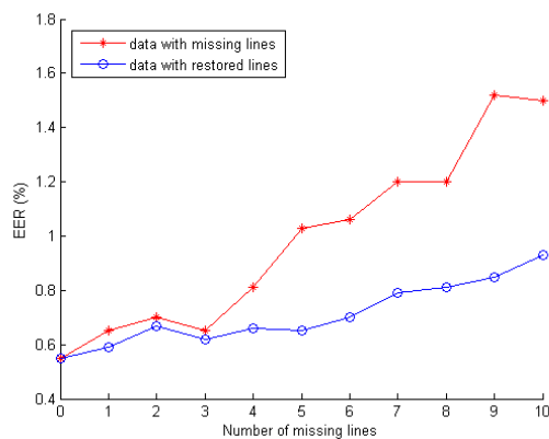
Figure 4: EERs obtained by using data with missing and restored lines as function of the number of missing lines.
