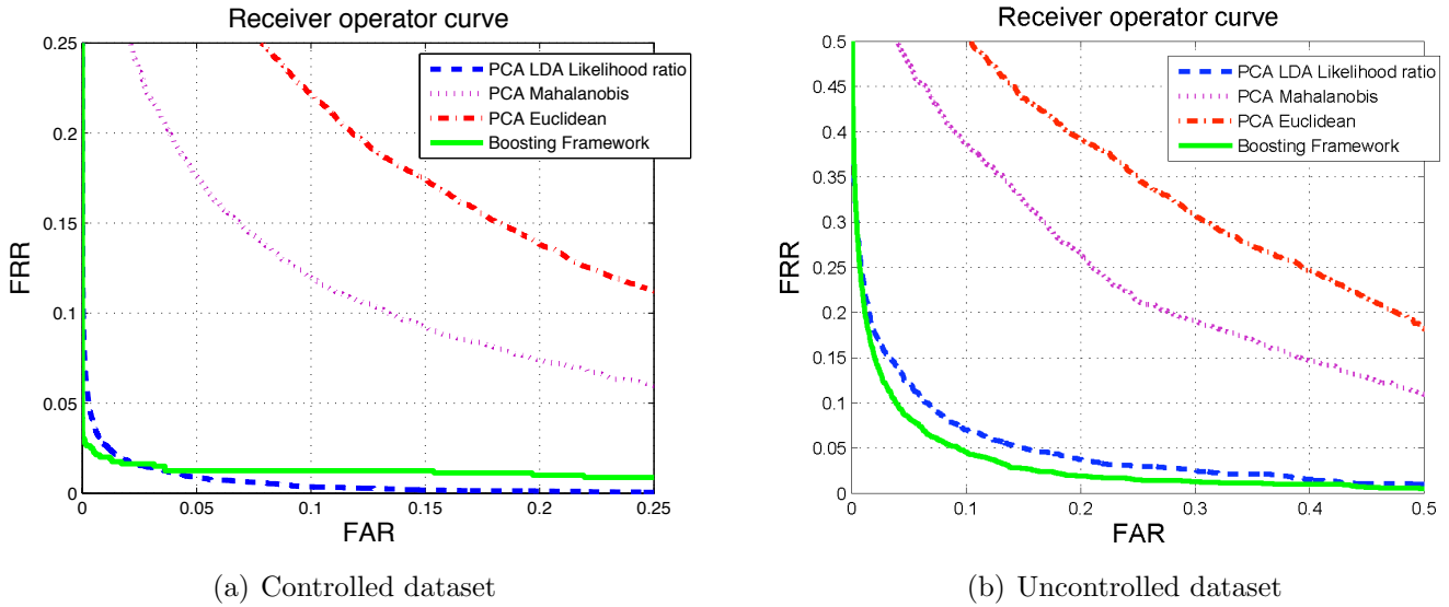
Figure 5: ROC on the subsets of the FRGCv1 database
