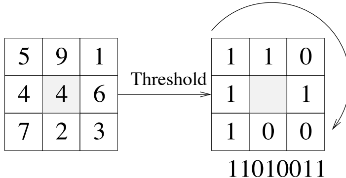
Figure 2: Local Binary Features
