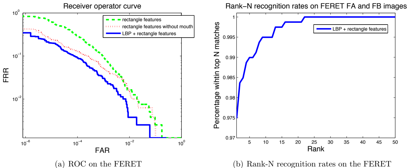
Figure 4: ROC and Rank-N recognition rates on the FERET FA and FB images of the boosting framework
